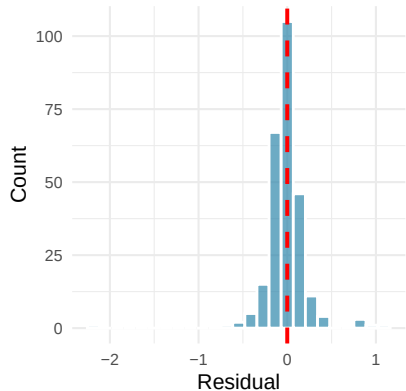
Residual Distribution
