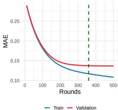
Learning Curves
