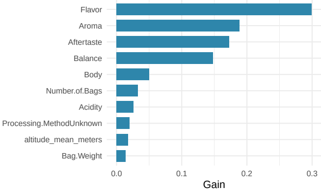
Top 10 Features by Gain
