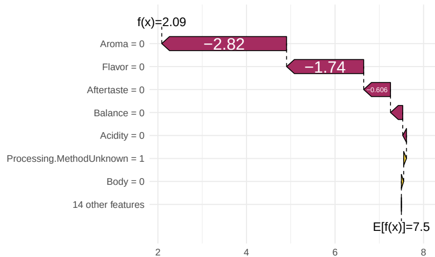
XGBoost: Flavor = 0
