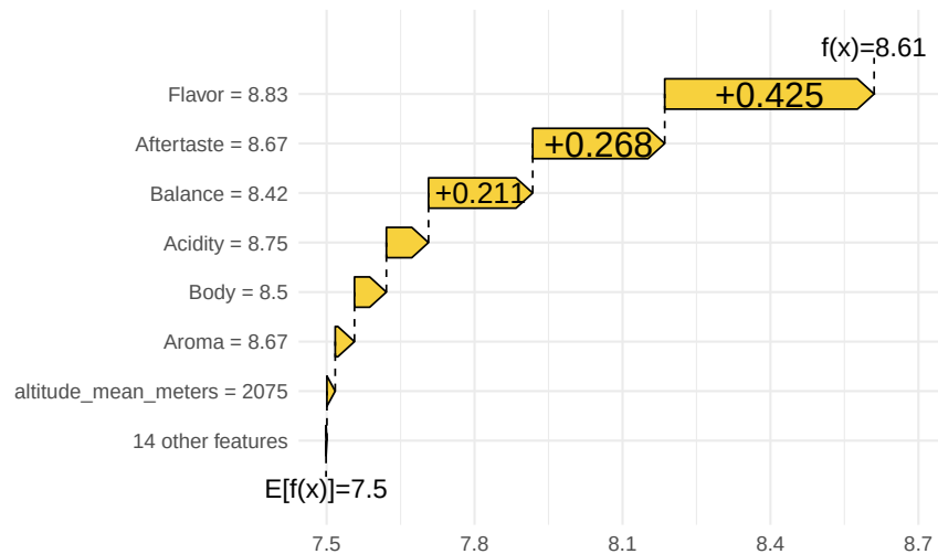
XGBoost: Flavor = 8.83
