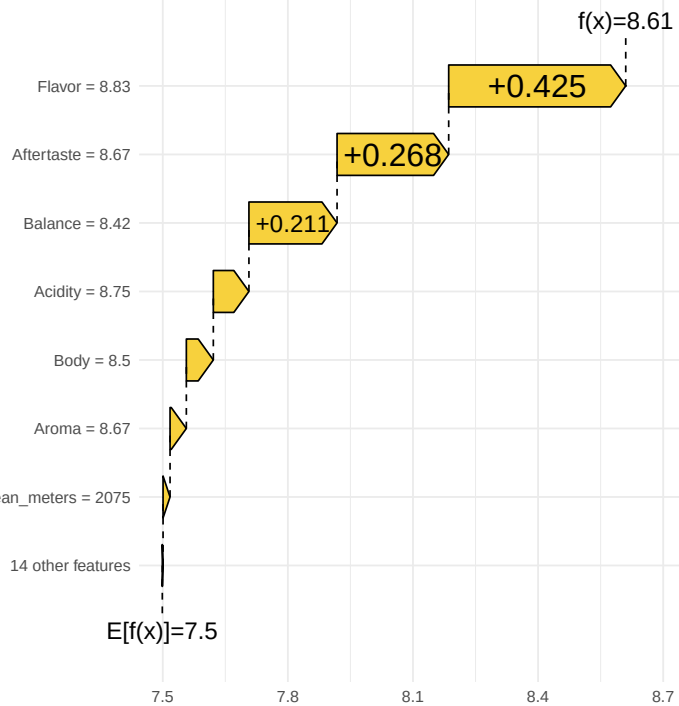
Waterfall Plot (XGBoost) Highest Flavor
