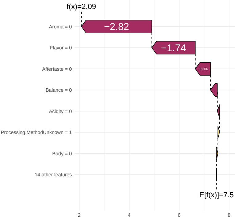
Waterfall Plot (XGBoost) Lowest Flavor
