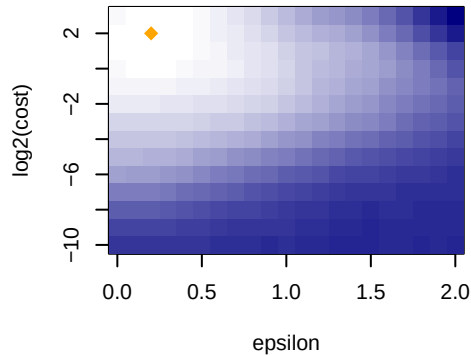
Errors using Radial Kernel
