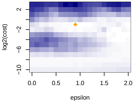
Errors using 2nd Degree Polynomial Kernel
