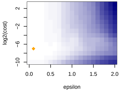
Errors using Linear Kernel
