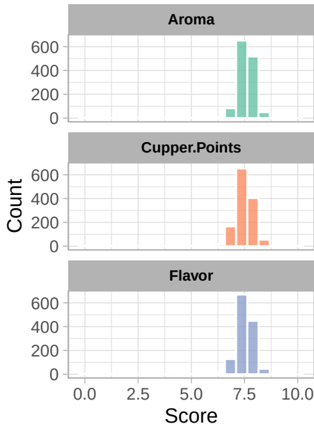
Distribution Shapes
