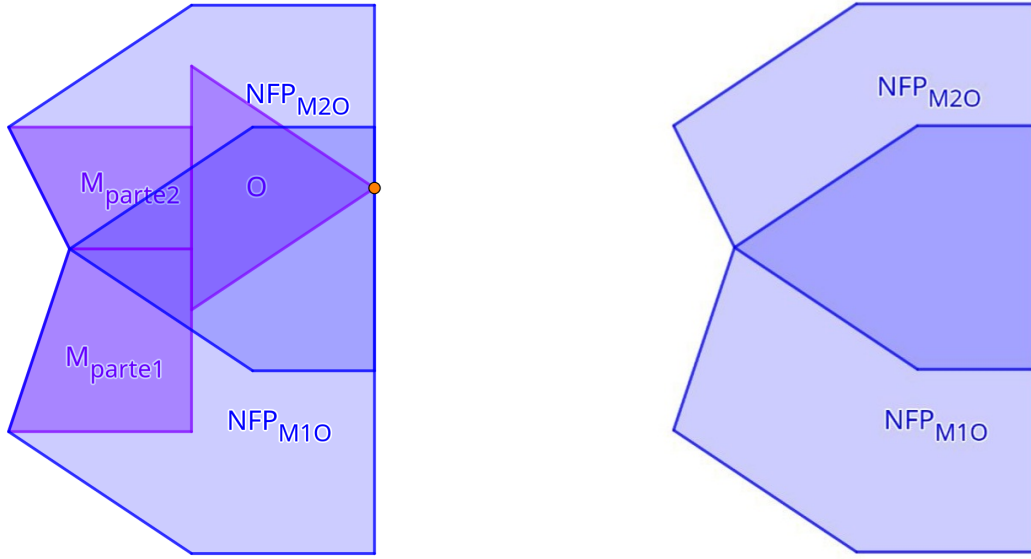
(a) Partes de M , O e as partes de NFP_{MO} .
