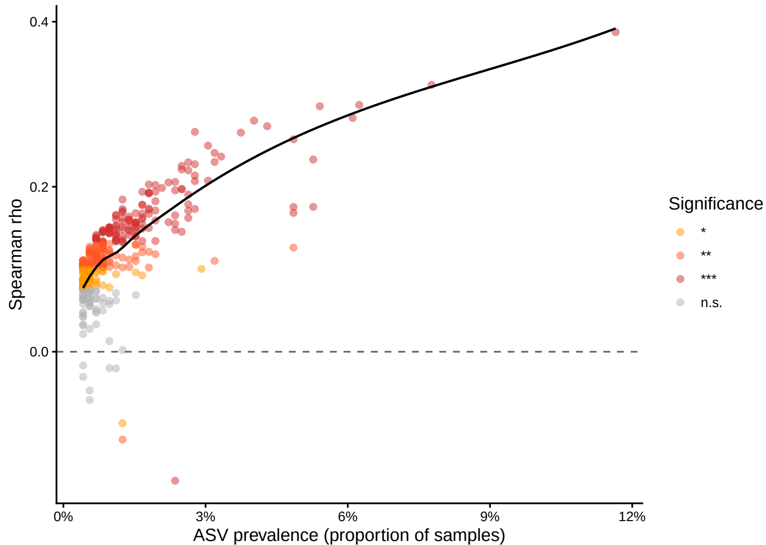
Co-occurrence strength vs. ASV prevalence
