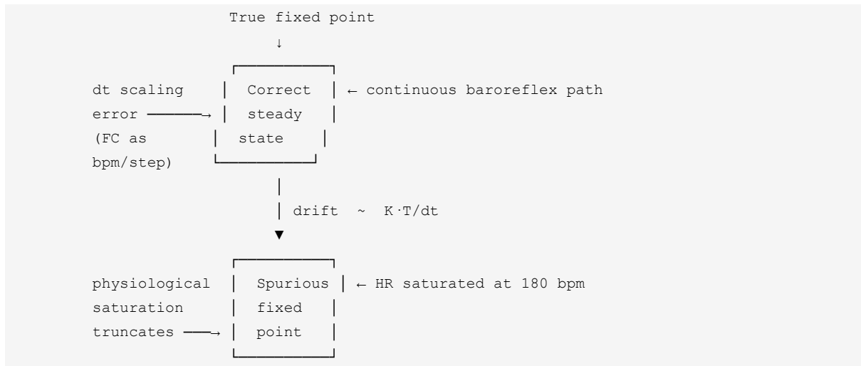
Figure 1: Spurious steady state schematic. The true fixed point is destabilized by the dt-dimensional error; saturation creates a false steady state.
