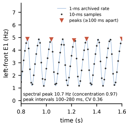
E Control 4: detector resolution (set 42, left-front E1)
