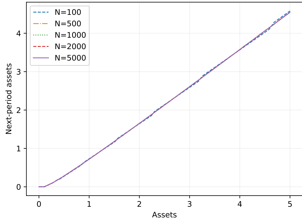
Part (g): next-period assets, exp_log grid on [0,5]
