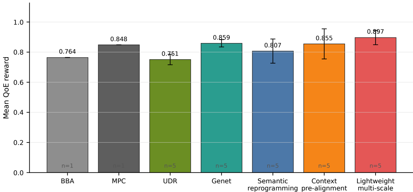
Overall ABR performance on FCC traces
