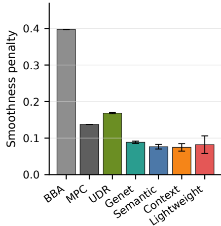
Smoothness penalty
