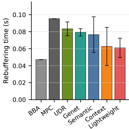
Rebuffering time
