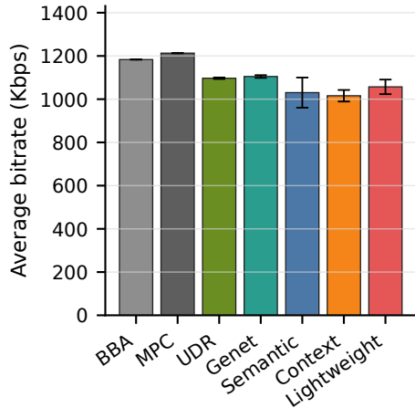
Average bitrate
