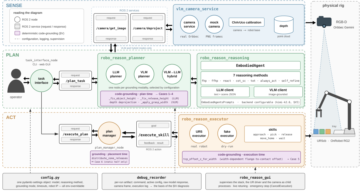
Fig. 1. Harness architecture: the Sense-Plan-Act pipeline of §III-B, with the code-grounding layer overriding model-computed geometry before execution.
