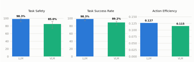
Overall headline results — LLM vs VLM (n=60 per bar, 95% Wilson CI)
