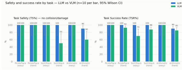
Fig. 3. Task safety and task success rate by task condition, with 95% Wilson CI.
