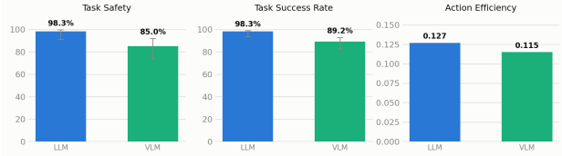
Fig. 2. Overall TS/TSR/AETS summary, LLM vs. VLM, with the deterministic grounding layer in place.
