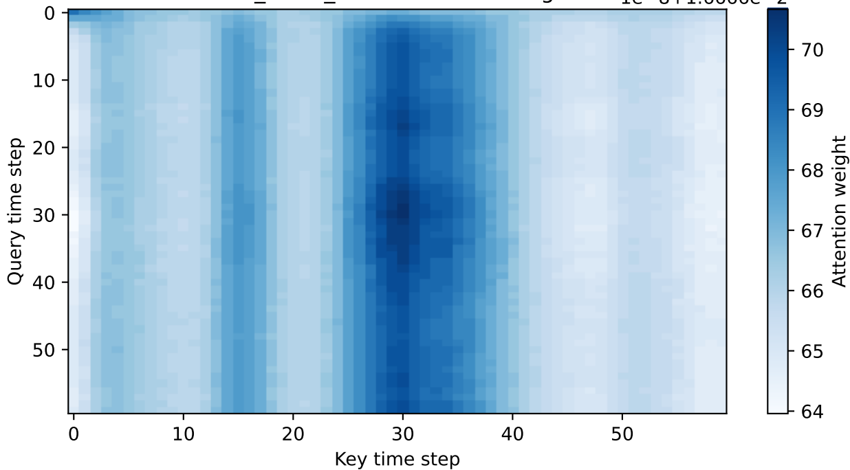
CNN_LSTM_Attn: attention weights
