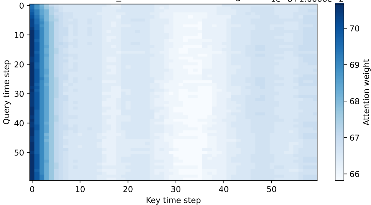
LSTM_Attention: attention weights
