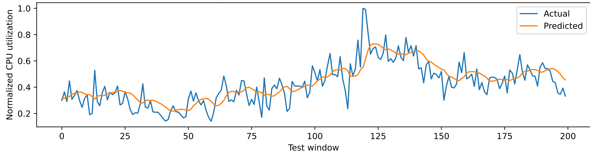
LSTM_Attention: 1-step-ahead forecast vs actual
