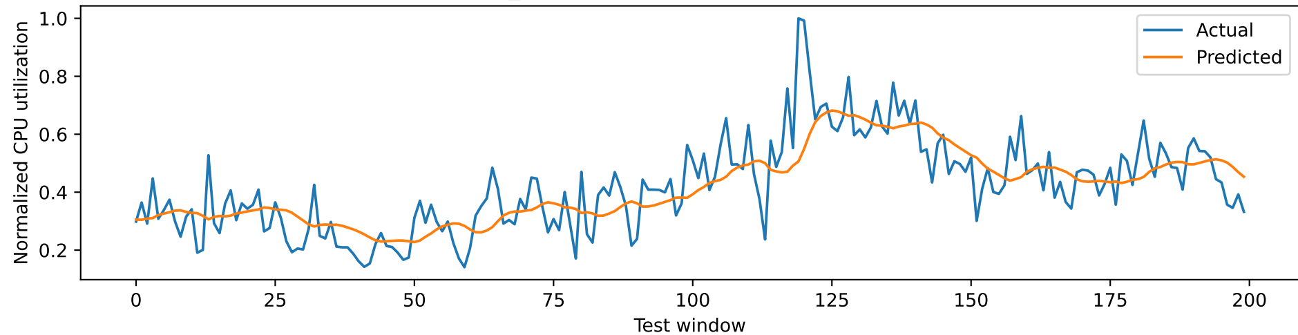
LSTM_only: 1-step-ahead forecast vs actual
