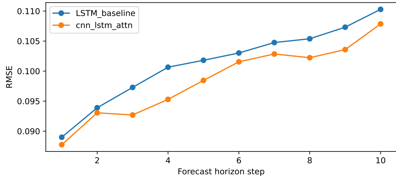
Forecast Error vs Horizon
