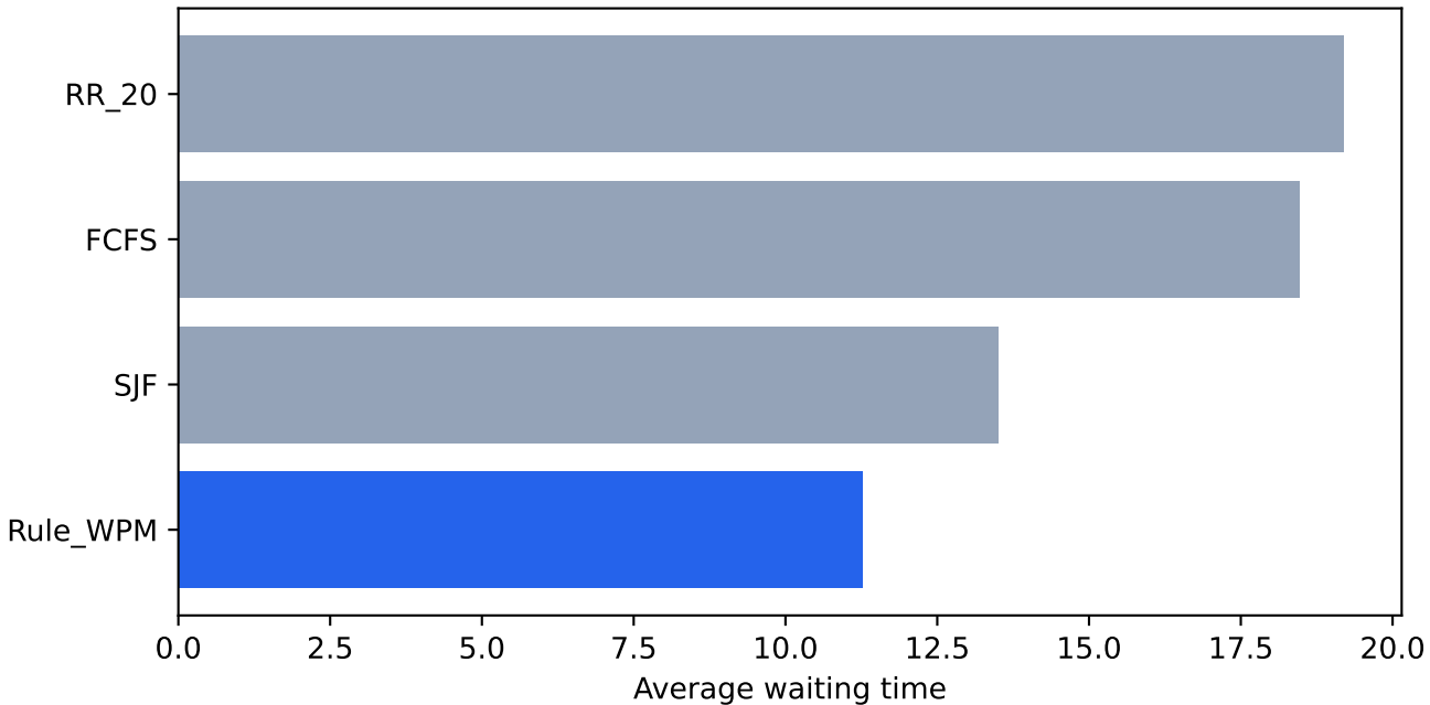
Scheduling Baselines vs Forecast-Aware Rule Advisor
