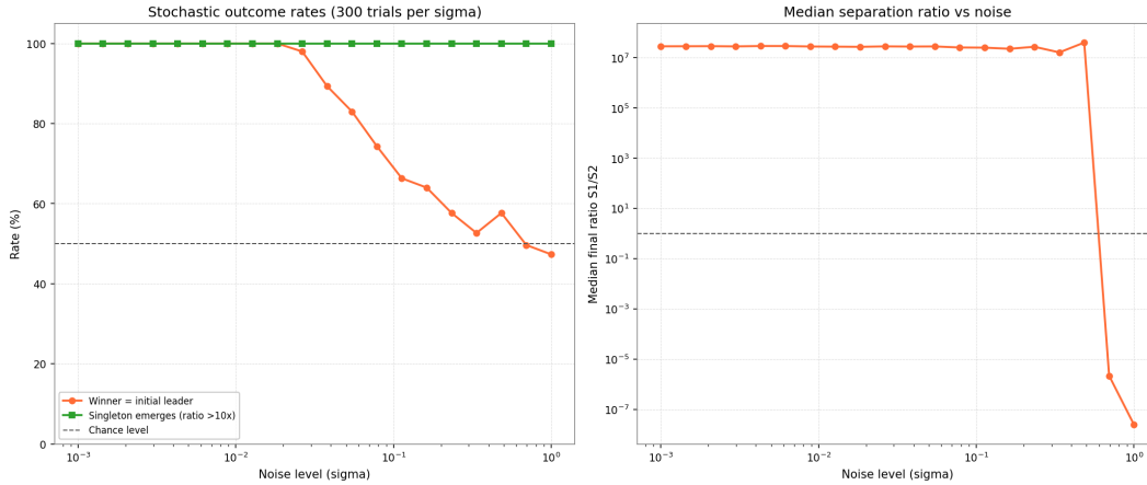
Figure 2: Stochastic simulation outcomes, 300 trials per noise level \sigma , integration cap at S = 10^8 . “Singleton emergence” counts trials reaching the cap (ratio > 10\times ) within t_{\text{max}} ; with the cap in place, no trials in the tested range fail. Winner identity: initial leader wins > 50\% of trials below \sigma \approx 0.23 (default 10% gap); degradation begins near \sigma \approx 0.023 . This is consistent with high \Pr(J \geq c) in Theorem 7.1 for small \sigma , not evidence of almost-sure emergence.
