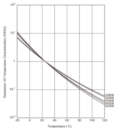
Resistance-Temperature Characteristics
