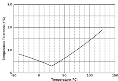
Temperature Tolerance VS. Temp.
