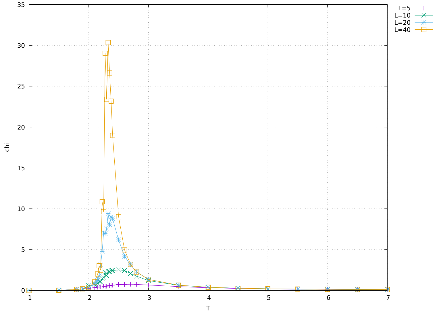
Magnetic susceptibility per spin
