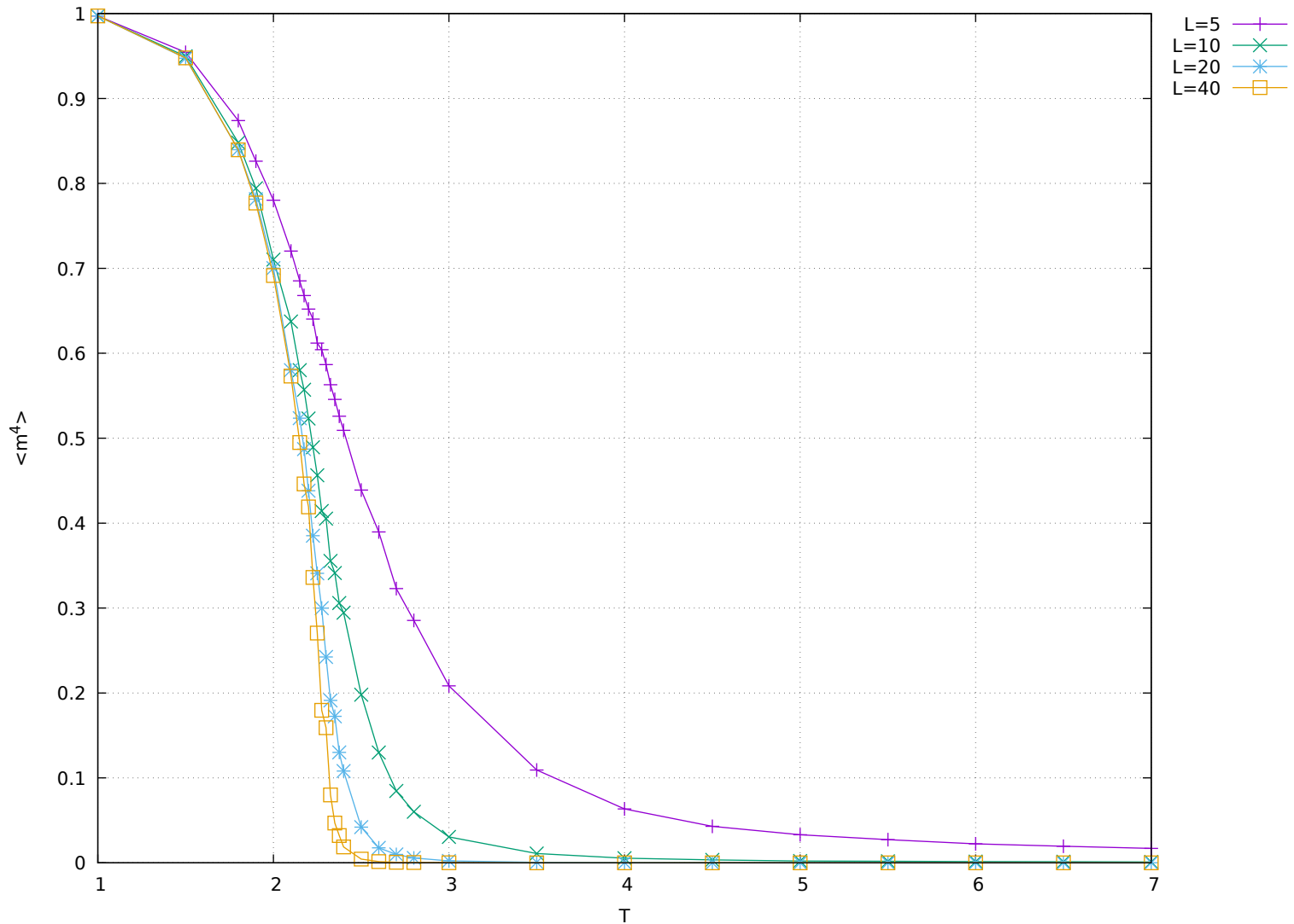
Fourth moment of magnetization
