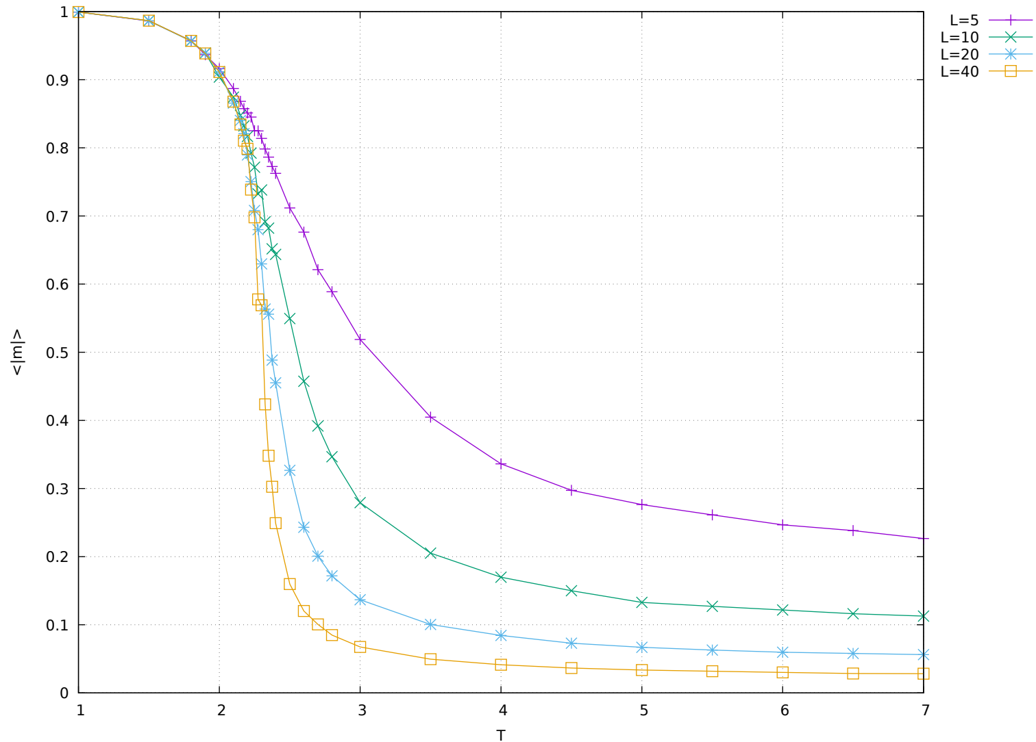
Absolute magnetization per spin
