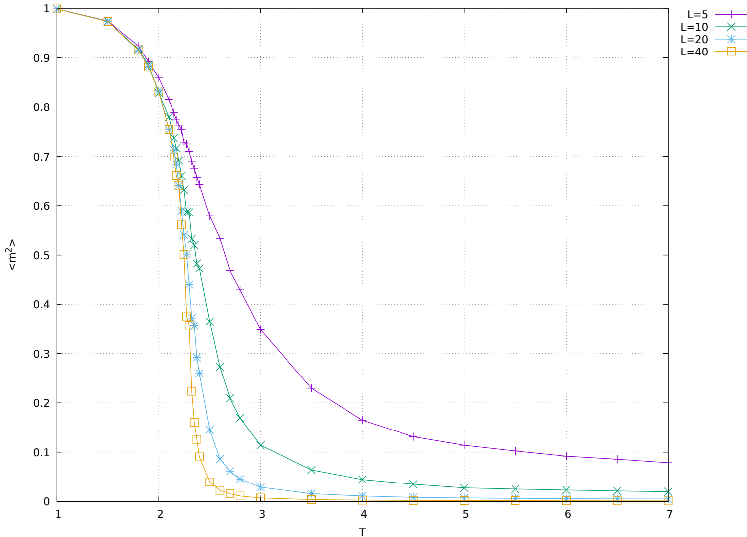
Second moment of magnetization
