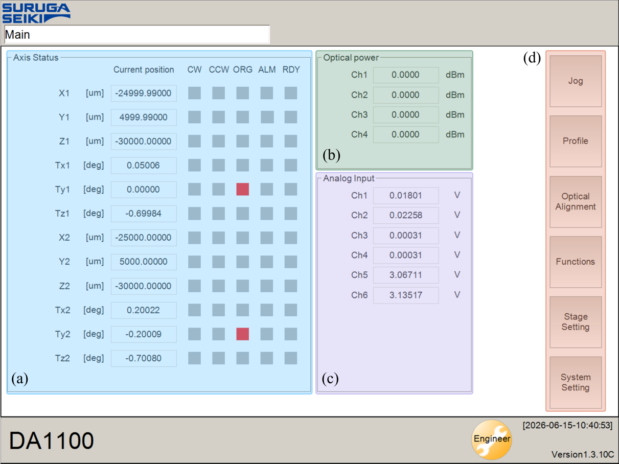
Figure 1.1: Main screen of the Suruga positioning system. The interface is divided into four main sections: (a) Axis Status, which displays the current position and status of each axis; (b) Optical Power, which displays the optical power measured by the connected power meter; (c) Analog Input, which displays the voltage measured at each available analog input channel; and (d) Function Access, which provides direct access to the main functionalities and configuration options of the Suruga platform.
