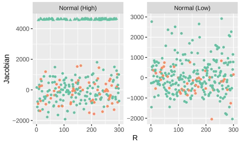
Jacobian
