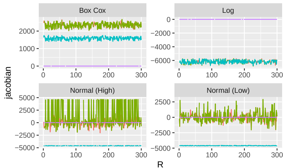
Jacobian
