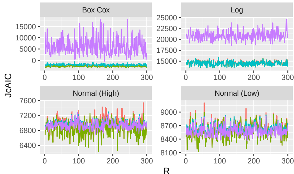
Jacobian
