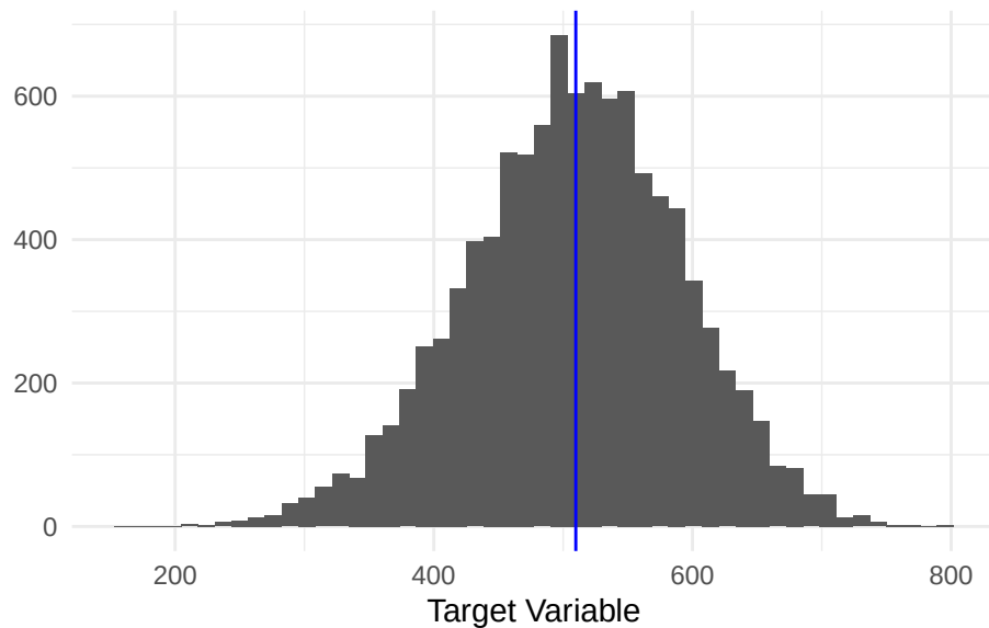
Normal (Low)
