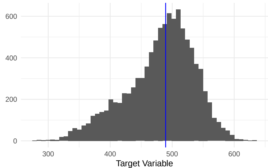
Normal (High)
