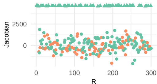
Jacobian
