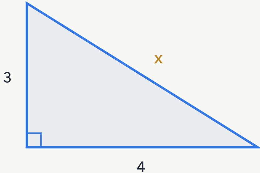
A right triangle
