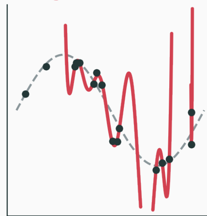
degree 15 — overfit
