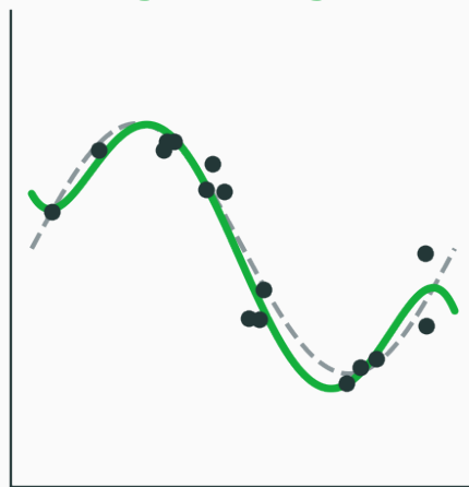
degree 5 — good
