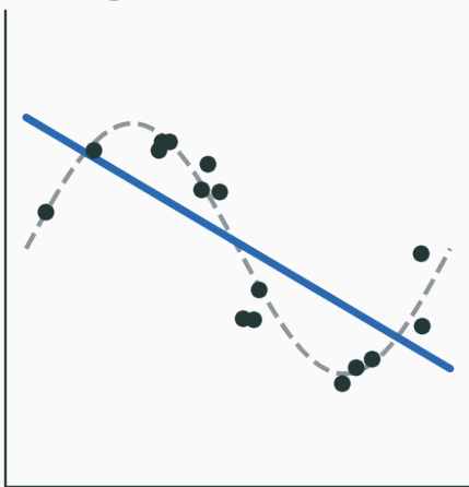
degree 1 — underfit
