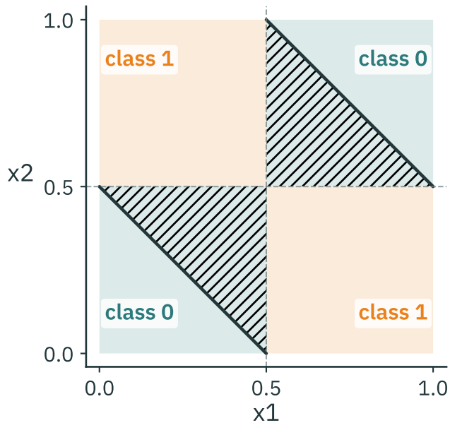
filled XOR regions: same rule misses areas
