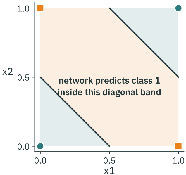
four Boolean inputs: all correct
