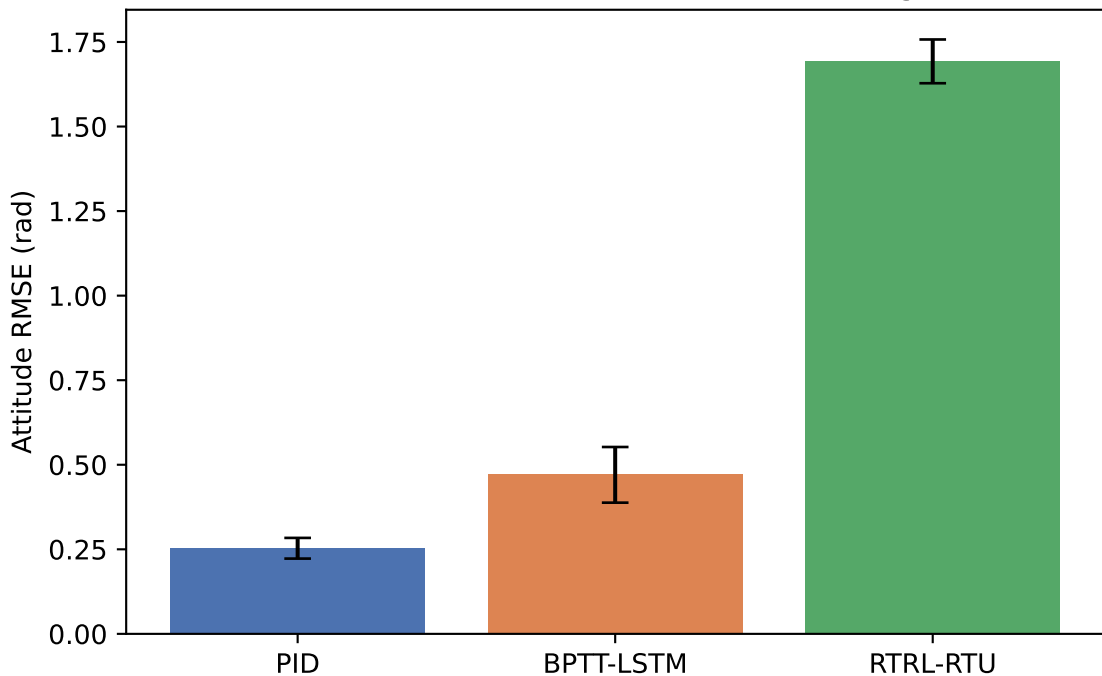
Combined Scenario: Attitude Tracking
