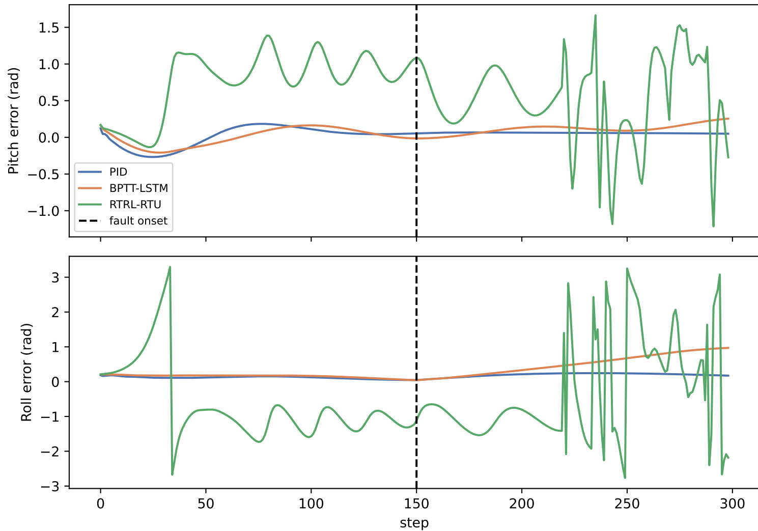
Fault Recovery: Tracking Error Over Time (seed=0)
