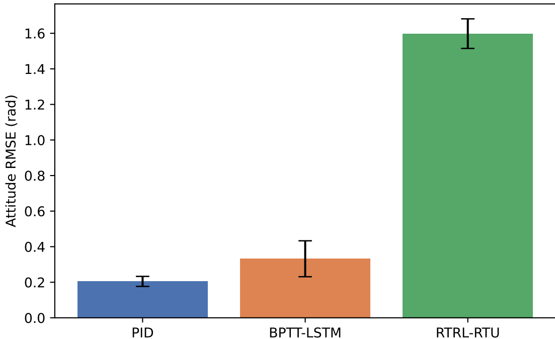
Wind Scenario: Attitude Tracking
