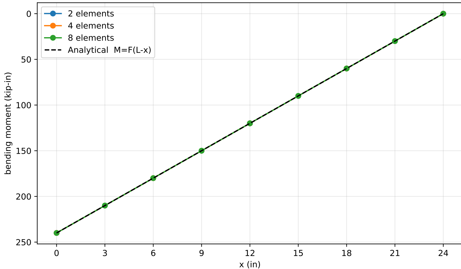
Bending Moment Diagram - mesh comparison
