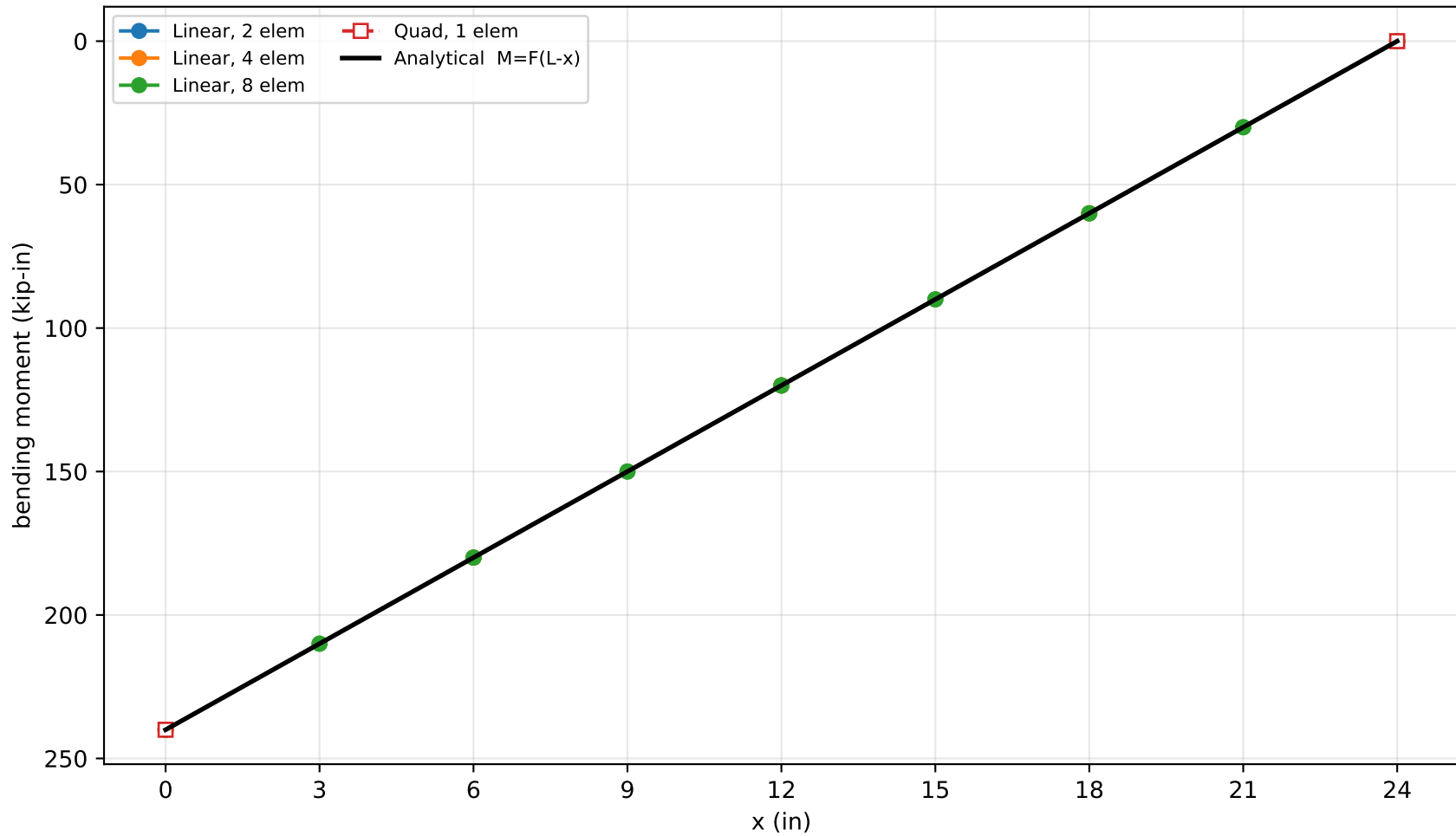
Bending Moment Diagram - linear vs quadratic
