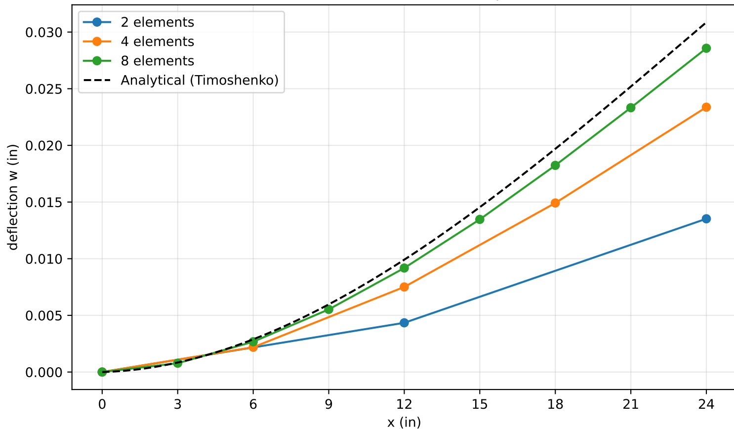
Vertical deflection - mesh comparison
