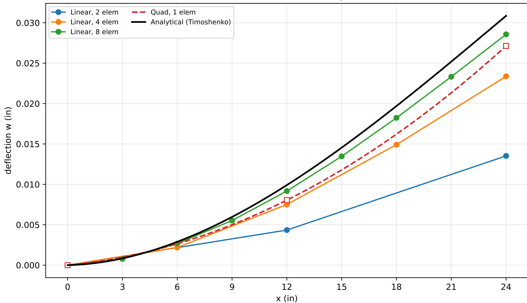
Vertical deflection - linear vs quadratic
