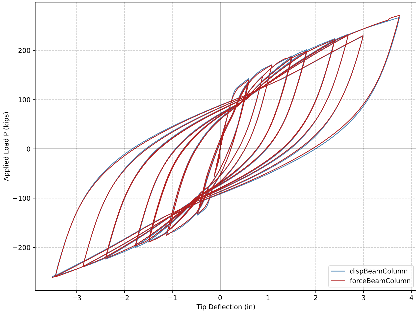
Hysteresis Curve
