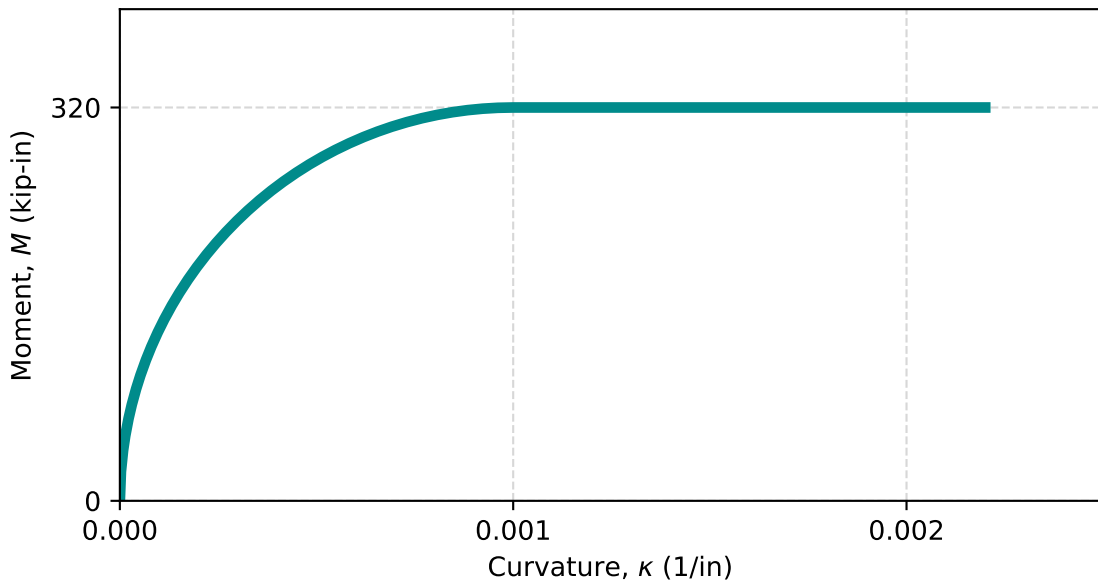
Moment-Curvature Relation
