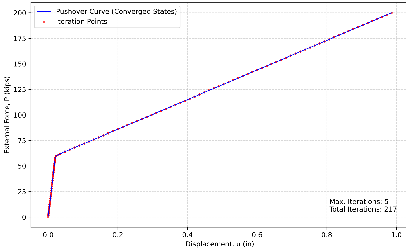
Part (a): Monotonic Pushover Analysis (Newton-Raphson)
