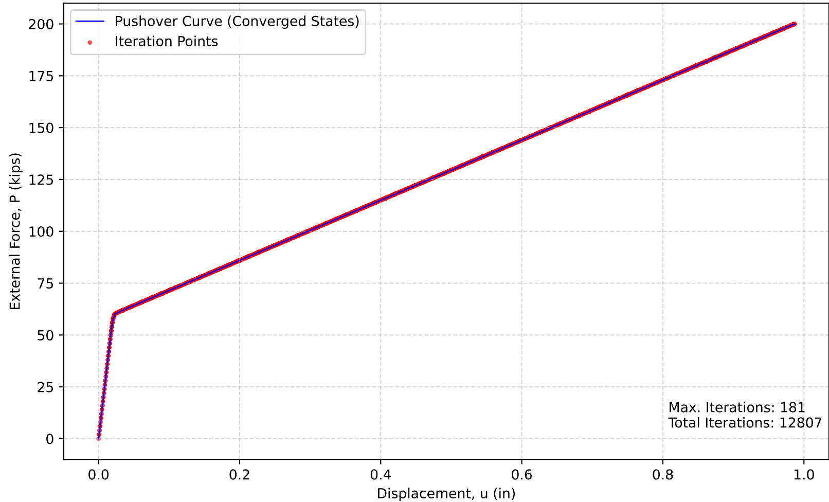
Part (b): Monotonic Pushover Analysis (Modified Newton-Raphson)
