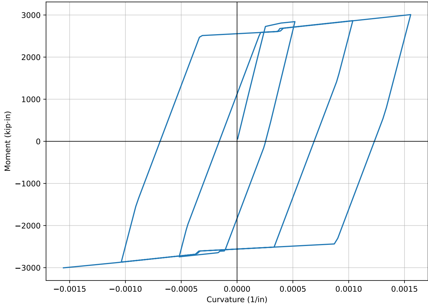
Moment-Curvature Diagram (Steel 01-Concrete 01)
