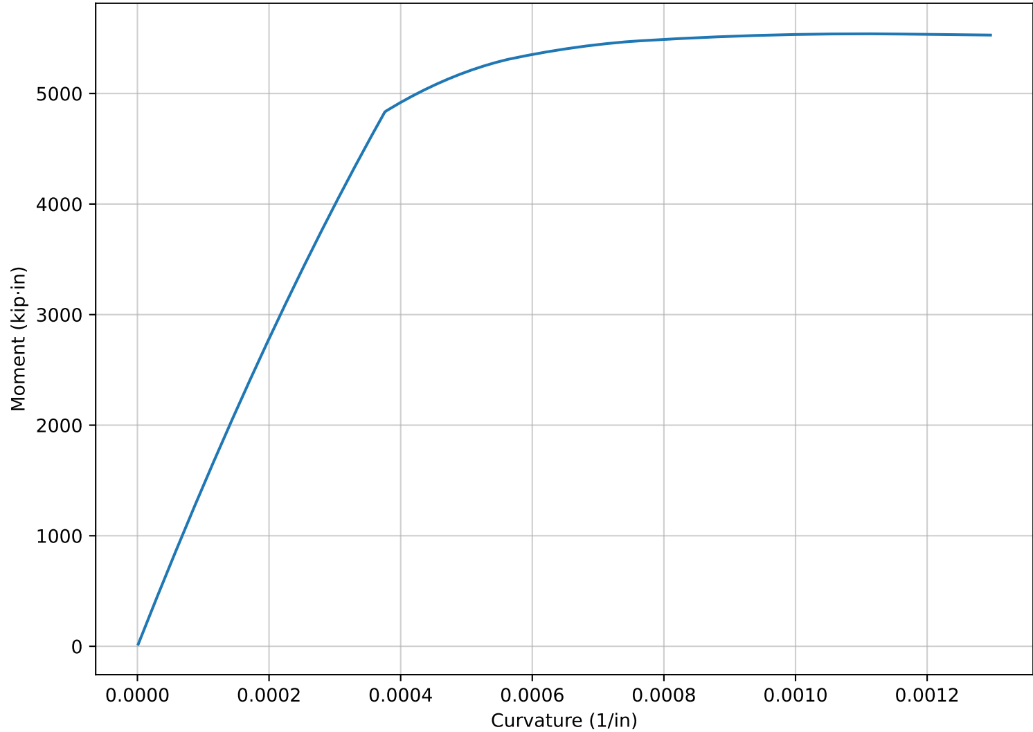
Moment-Curvature Diagram (Monotonic, Displacement Controlled, fixed Axial DOF)
