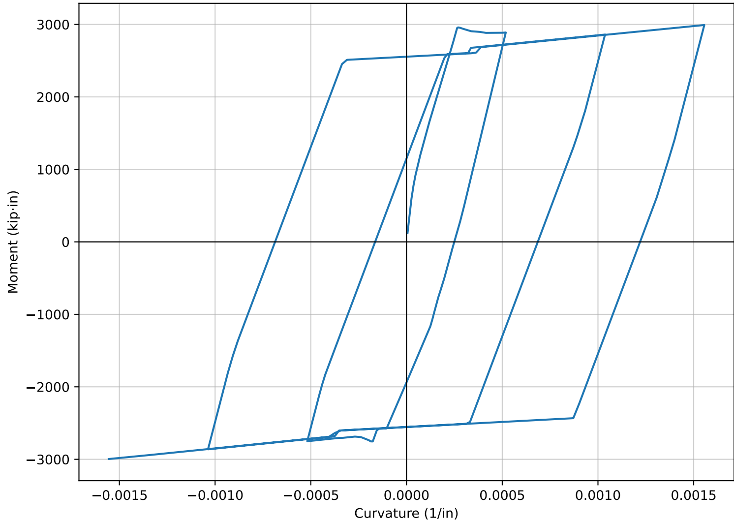
Moment-Curvature Diagram (Steel 01-Concrete 02)
