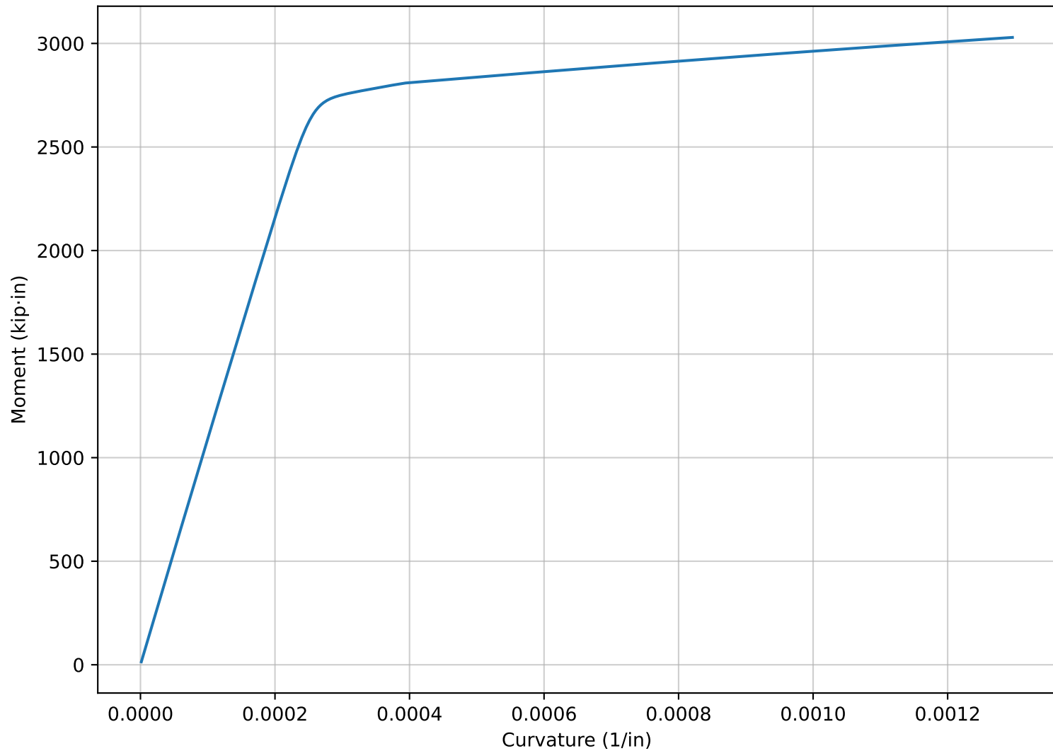
Moment-Curvature Diagram (Monotonic, Displacement Controlled)
