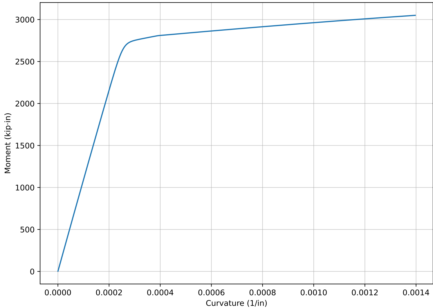
Moment-Curvature Diagram (Monotonic, Load Controlled)
