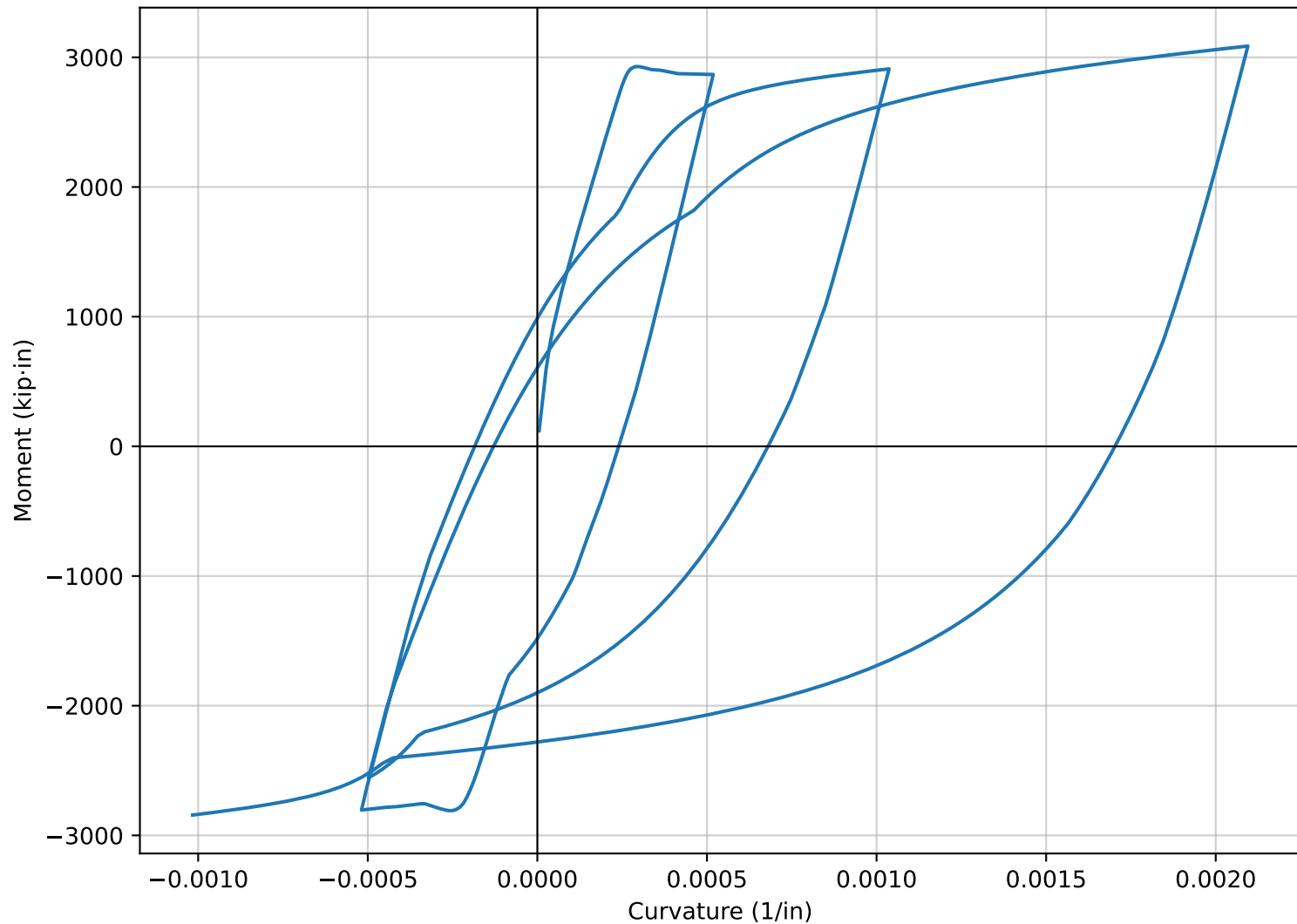
Moment-Curvature Diagram (Steel 02-Concrete 02) (Modified Newton)
