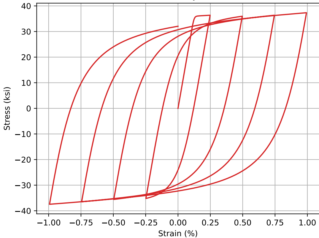
Stress-Strain Hysteresis
